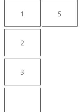
LoginAttempts
